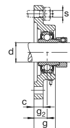
FL362
