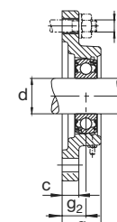
FL762..2RSR
