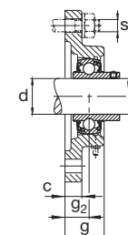
FL562
