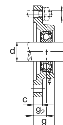
FL762..2RSR
