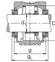
Anel labirinto TSV
