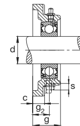
F762..2RSR
