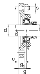
FL162
