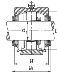
Anel labirinto TSV
