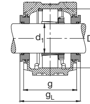
Anel labirinto TSV
