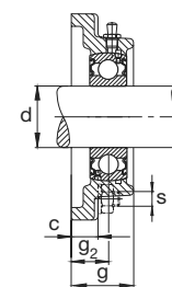
F762..2RSR
