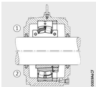
Locating bearing S30
